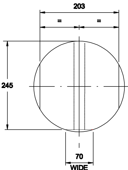
PLAN DETAIL 'A'
