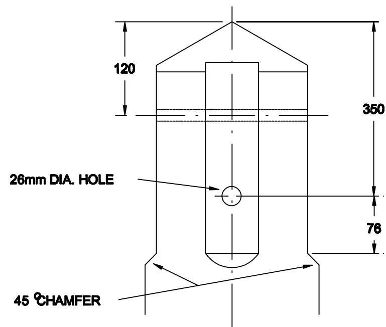
SIDE ELEVATION ON VIEW 'A' & 'B' SCALE 1:5
